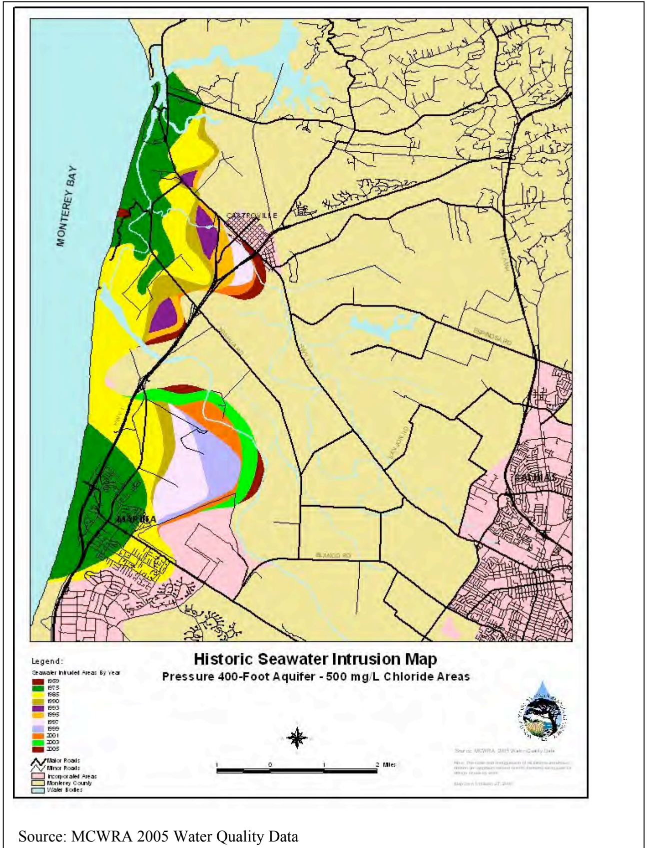
Figure 2.2 Saltwater Intrusion in Monterey County's 400-Foot Aquifer
