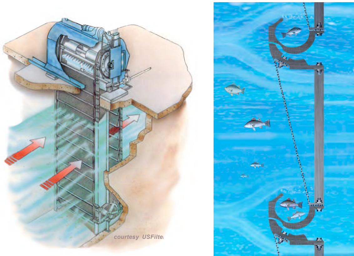
Figure 5.4. Ristroph Traveling Screen
