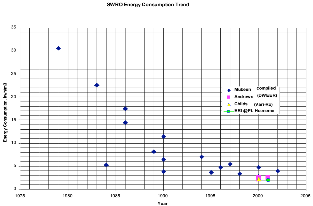
Figure 4.9 Seawater Reverse Osmosis Energy Consumption Trend
