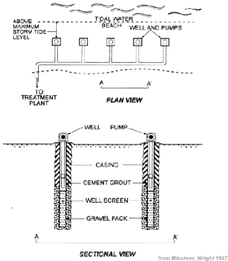
Figure 5.1. Vertical beach wells
