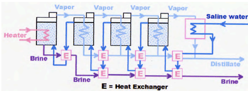
Figure 4.3. Multiple Effect Distillation
