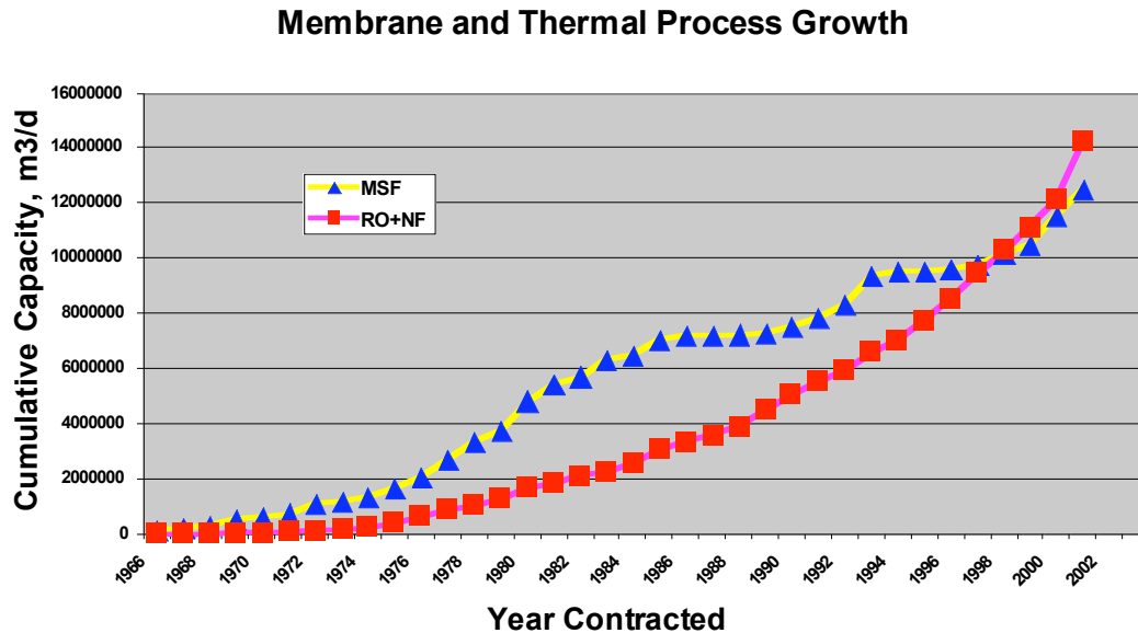
Figure 4.1 Membrane and Thermal Process Growth
