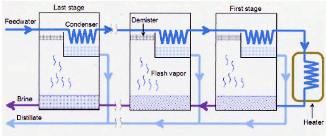
Figure 4.2: Multi Stage Flash Evaporation
