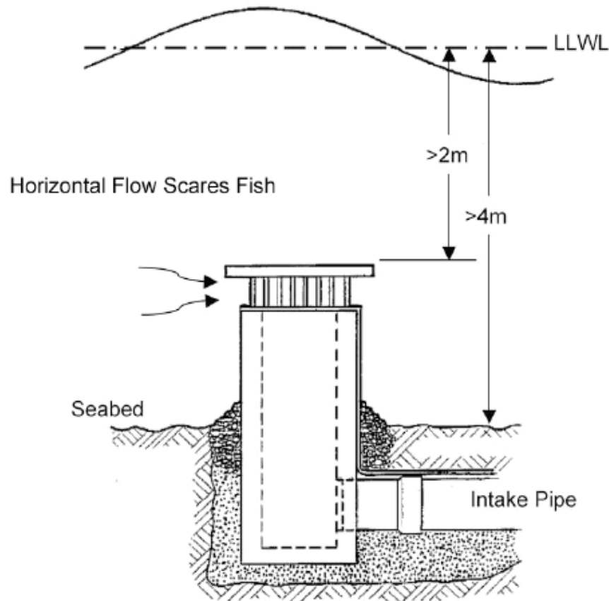
Figure 5.6 Velocity cap
