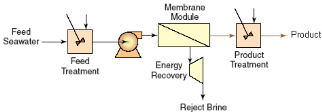
Figure 4.6 Reverse Osmosis Process
