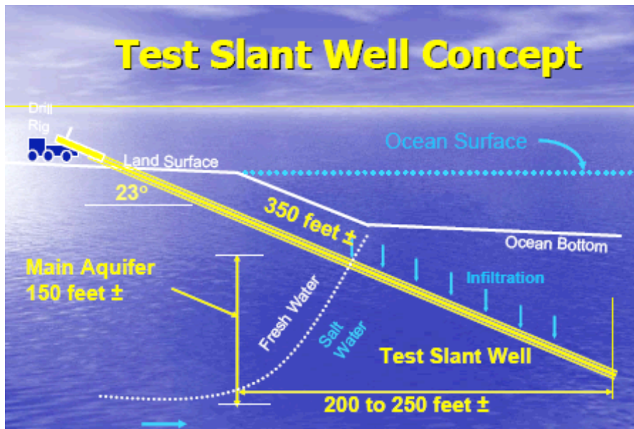
Figure 5.3. Dana Point slant well (MWDOC Prop 50 proposal, 2006)
