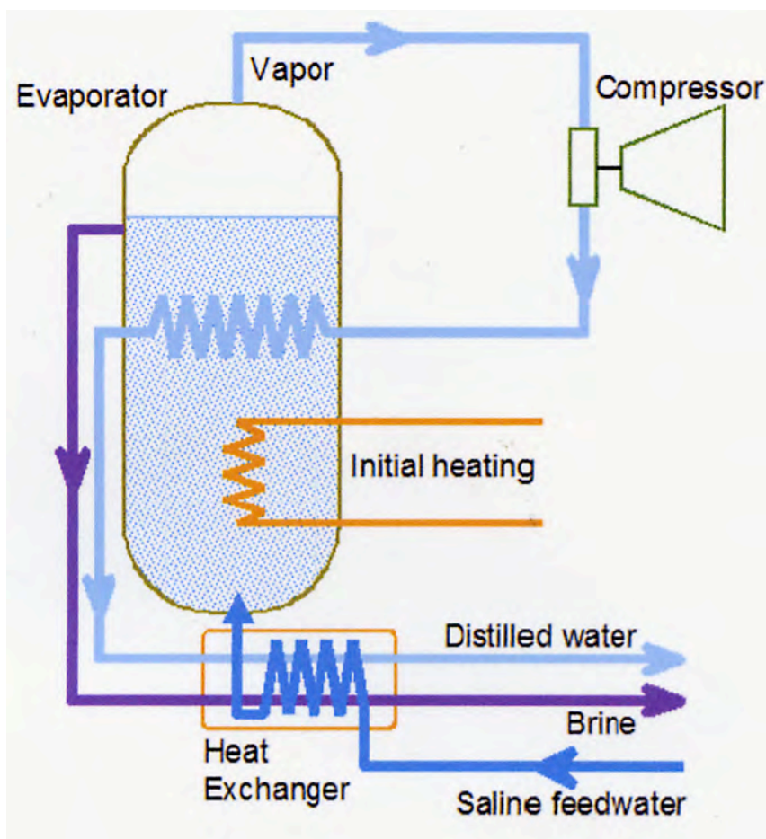
Figure 4.4: Vapor Compression Distiller
