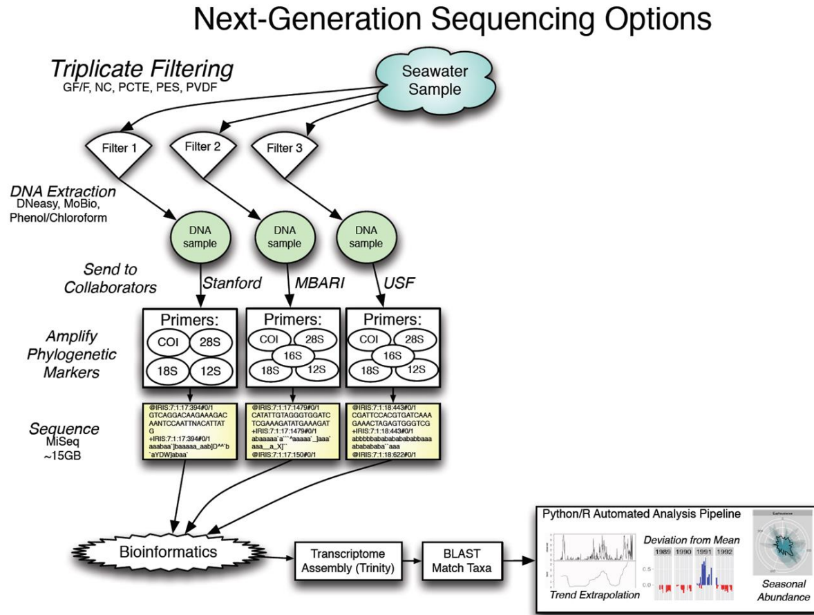
Fig. 3. Summary of MBON genomic/eDNA sampling and analyses.
