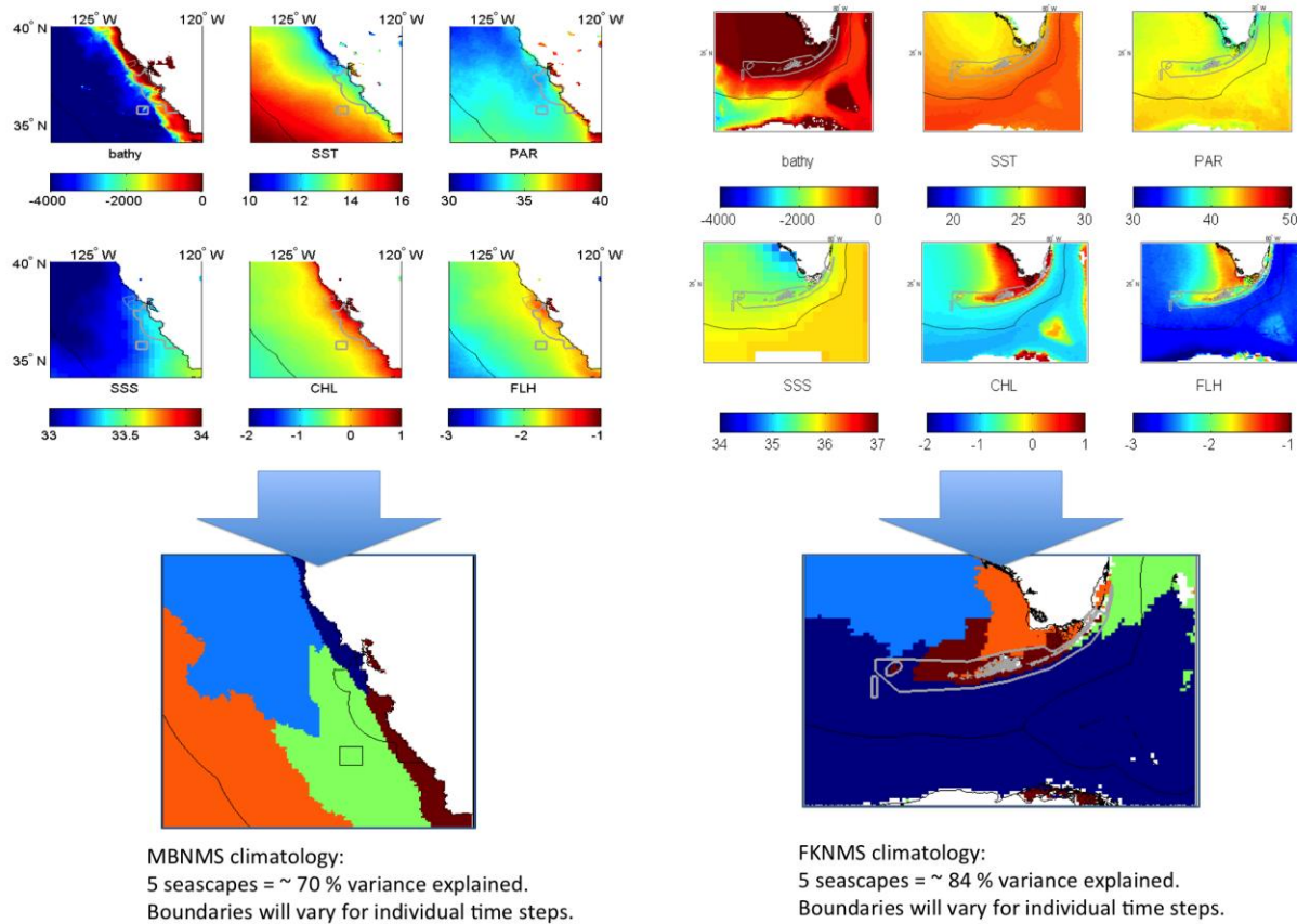
Figure 4. Seascape climatologies (2003-2008) for the FKNMS and MBNMS are shown in panels indicated by the blue arrows. The seascape distributions at each Sanctuary are derived from biophysical variability of parameters shown above the seascape panels (bathymetry, sea surface temperature (SST), photosynthetically active radiation (PAR), sea surface salinity (SSS), chlorophyll-a (CHL), and fluorescence line height (FLH).
